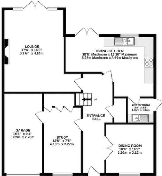
GROUND FLOOR 963 sq.ft. (89.4 sq.m.) approx.
